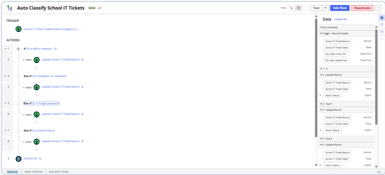
Figure 2: Published Auto Classify School IT Tickets Flow Designer workflow showing keyword condition branches.
